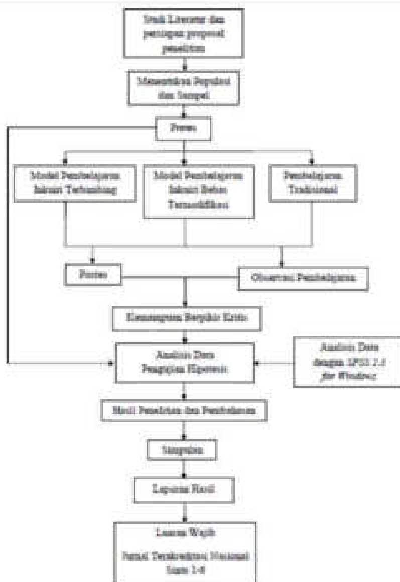
Gambar 2. Alur Penelitian
